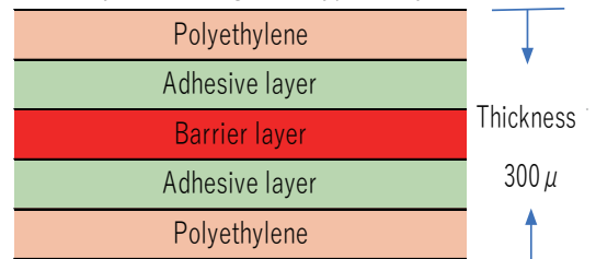
Multi-layer tube Diagram(4 types 5 layers)
